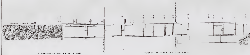
ELEVATION OF PART OF MASSIVE WALL EXPOSED TO EAST OF BIRKET ISRAEL N o 1 st
